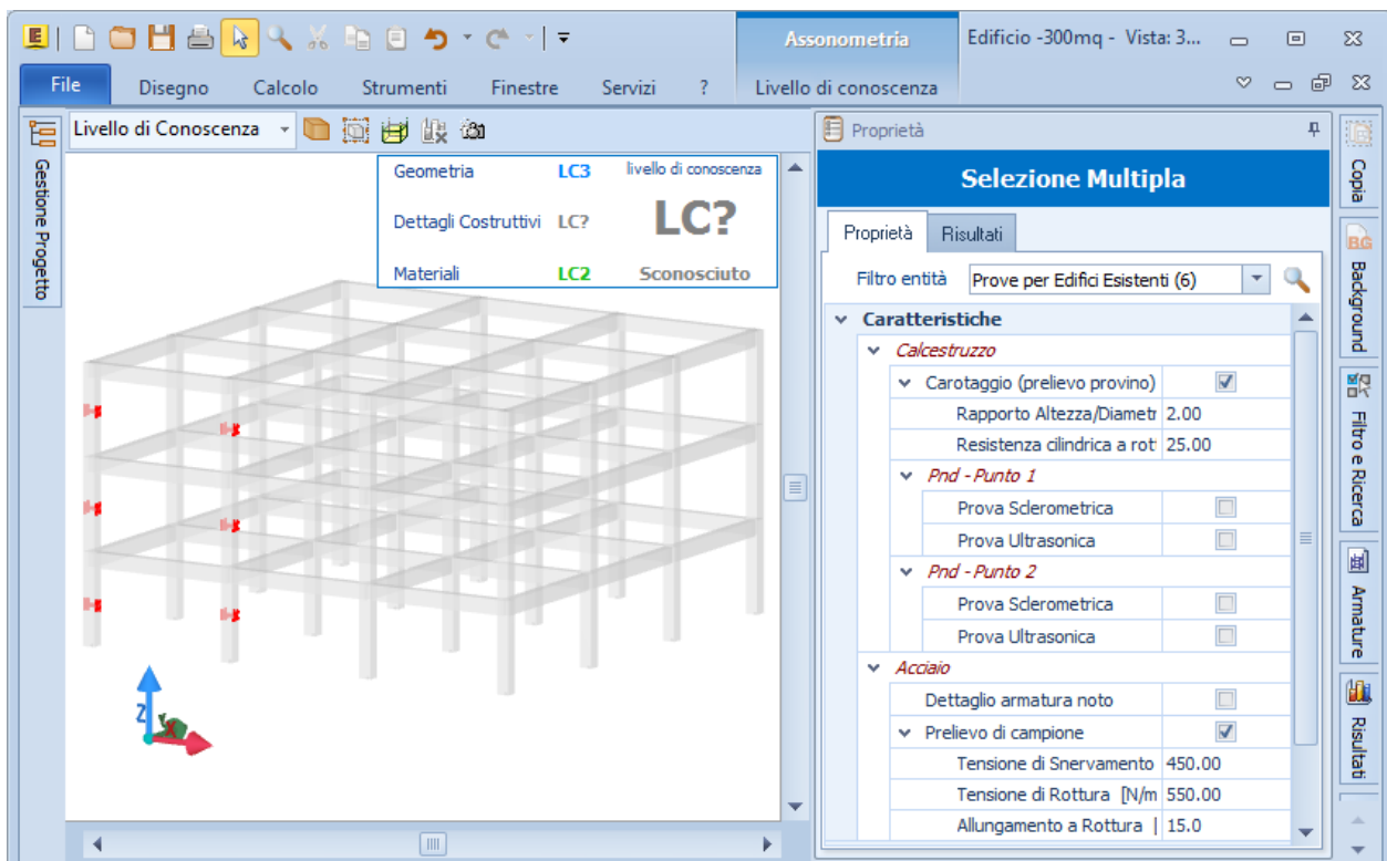
Figura 1.11: LC2 - Materiali
