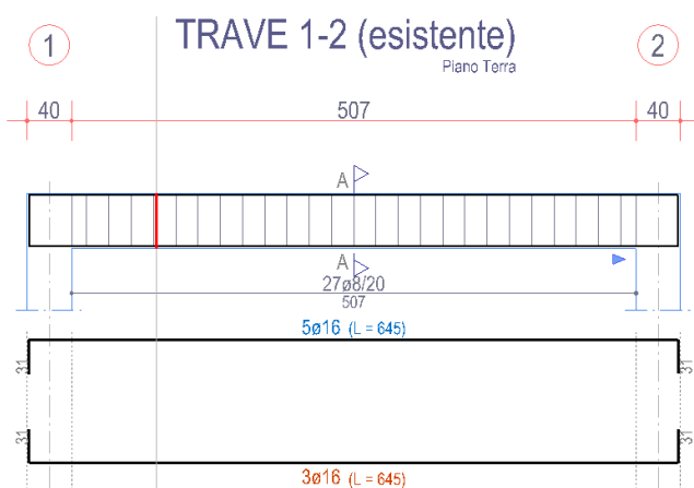
Figura 14.3: armature Trave 1-2
